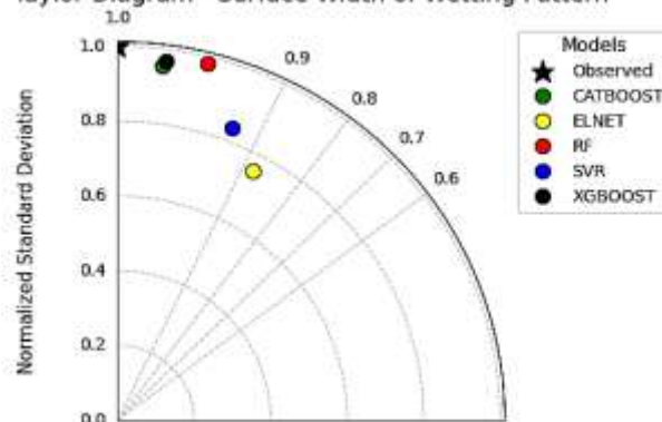
Taylor Diagram - Surface Width of Wetting Pattern
